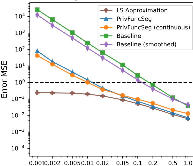
Degree-1 Monomial Basis
